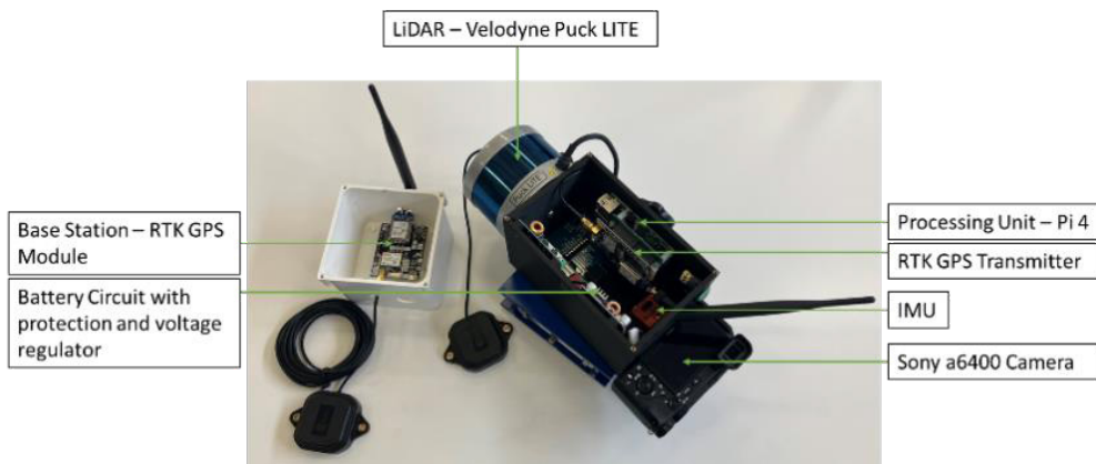
Fig. 2. Labeled sensor payload diagram.
