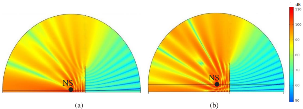
Fig. 6. The distribution of sound pressure levels over a rigid ground in the presence of the barrier with h_e=12 m at a frequency of 125 Hz with source at h_1=1 m (a) and h_1=4 m (b)
