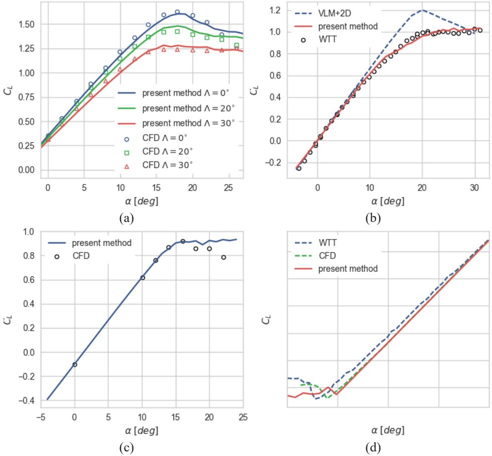
Fig. 5. Comparison of C_L - \alpha as computed by CFD or wind tunnel testing and the present method, for (a) three wings from [10] ( AR=12 , TR=1 , NACA 4416 profiles, Re=3 \cdot 10^6 , M=0.2 ), (b) the NACA TR1208 wing [11] ( AR=8 , \lambda=0.45 , \Lambda=45^\circ , NACA 631A012 profiles, Re=4 \cdot 10^6 ), (c) the Selena project geometry ( AR=5 , \lambda=0.35 , \Lambda=28^\circ , Re=4 \cdot 10^6 , M=0.2 ), and (d) the body-tail configuration.
