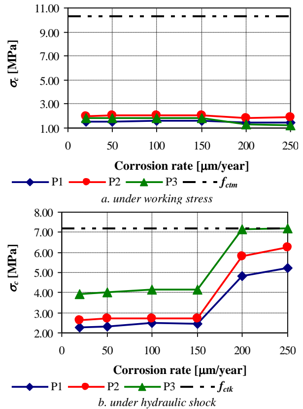
Fig. 8. Shotcrete longitudinal tensile stress with corrosion rate.
