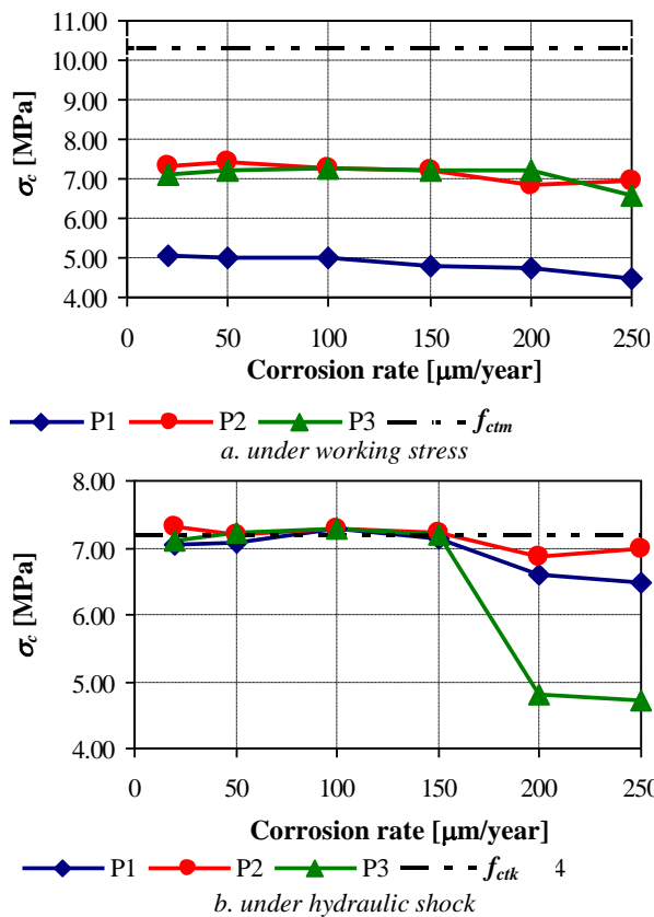
Fig. 7. Shotcrete radial tensile stress with corrosion rate.
