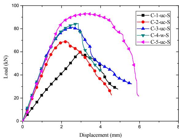
Fig.7. Load-displacement curves of Group C
