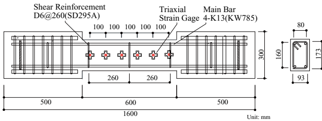
Fig 2. Configuration of specimens
