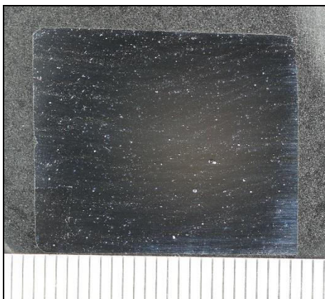
Fig. 6. Macro test specimen revealing fusion lines
