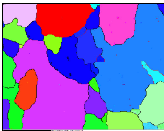
Fig. 9. Microstructure of plane normal to the torch progression of Wall-2
