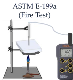
Figure 1. Experimental set-up of horizontal Bunsen burner fire test.
