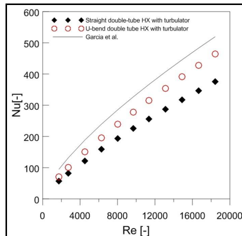
Fig. 7. Nusselt number at shell side for SDTHX and UBDTHX with helicoidal turbulator in single phase flow regime.
