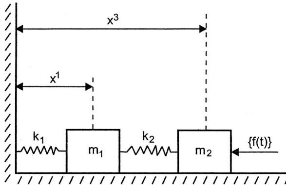
Fig. 2. Mechanical system [4].
