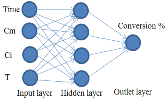
Fig. 1. Radial basis function neural network (RBFNN) structure.
