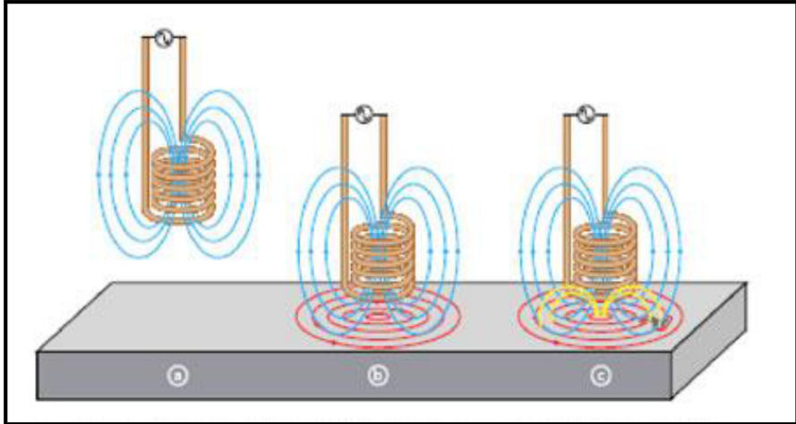
Figure. 1. Principle of Eddy Current Testing
