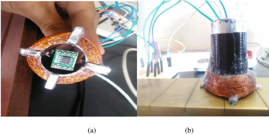
Figure. 5. GMR-coil probe; (a) bottom; (b) front
