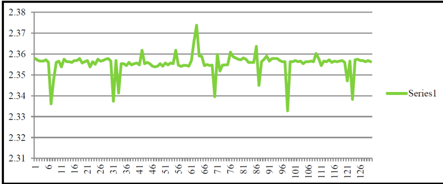
Figure. 7. Line graph for slot 0.5mm of brass calibration block
