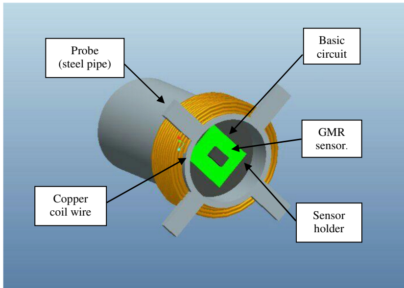
Figure. 4. Drawing for GMR-coil probe
