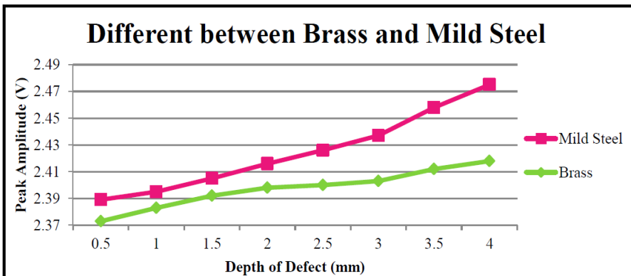
Figure. 9. Difference between brass and mild steel
