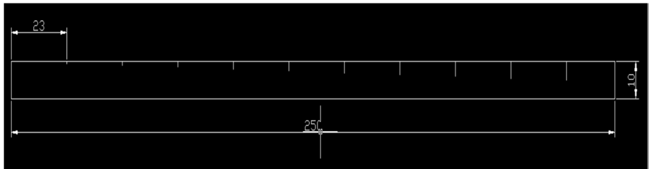
Figure. 3. Calibration block brass front view
