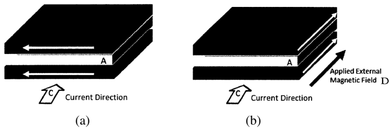
Figure. 2. a) GMR film layers without an applied magnetic field showing directions of magnetic moments b) GMR layers in the presence of an applied magnetic field.
