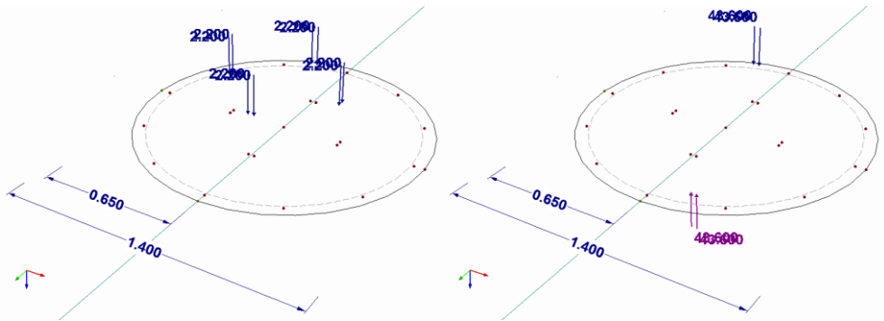
Fig. 6. Placement of the vertical forces ( N_F/8 \geq 2.2 kN) and overturning moment ( M_F/2 * 0.57 \geq 9.7 kN).
