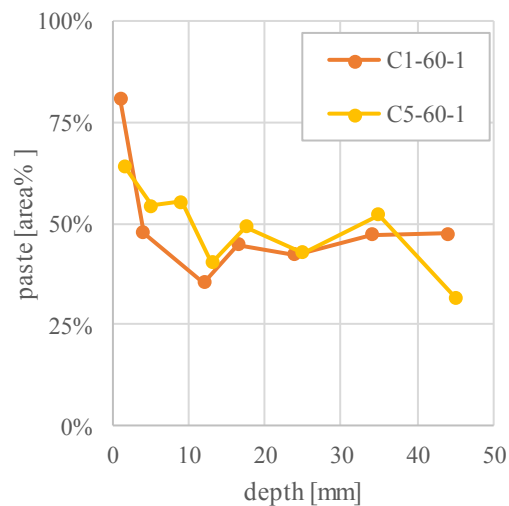
Fig. 14 : The area% of paste in the sections as a function of the depth from the surfaces determined using the phase differentiation with the \mu XRF.
