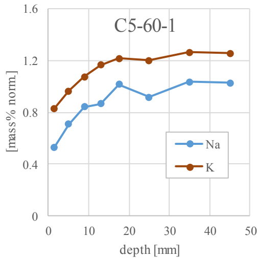
Fig. 12 : The elemental profiles for Na and K in the cement paste of the concrete sample C5-60-1 as a function of depth from the leached surface.
