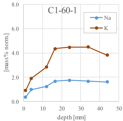
Fig. 11 : The elemental profiles for Na and K in the cement paste of the concrete sample C1-60-1 as a function of depth from the leached surface.
