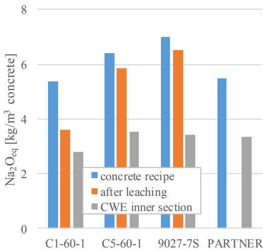
Fig. 15 : The \text{Na}_2\text{O}_{\text{eq}} content (in \text{kg/m}^3 of concrete) based on the concrete recipe (Table 2), the average alkali content in the sample after leaching, and the alkali content in the inner section of the concrete sample obtained by CWE.
