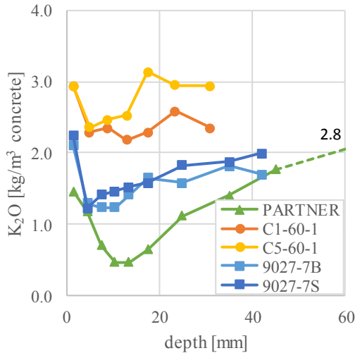
Fig. 8 : The K 2 O-profiles (in kg/m 3 concrete) in function of the depth of the exposed surface (in mm) obtained by CWE for the examined samples. The 2.8 kg/m 3 K 2 O indicated in the graph reflects the content determined on a section taken at a depth of approx. 100 mm-150.
