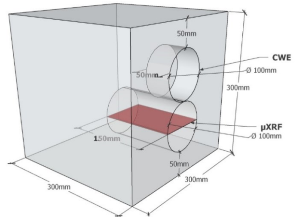
Fig. 1 : Sampling from the PARTNER cube.
