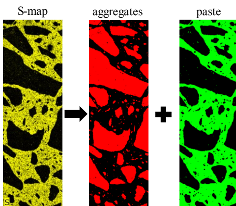
Fig. 6 : Demonstration of the differentiation between aggregates (red) and paste (green) in section 30-40 mm of sample C5-60-1 using the S elemental map.
