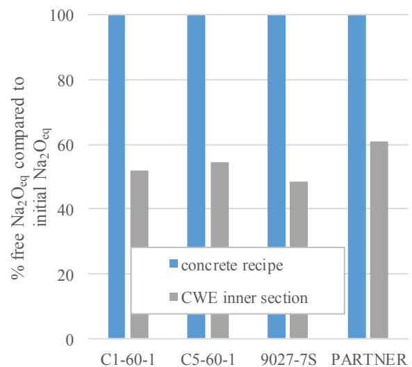
Fig. 17 : The share of the free alkali content left in the inner sections of the initial alkali content of the concrete (Table 2).
