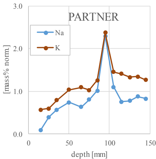
Fig. 13 : The elemental profiles for Na and K in the cement paste of the concrete sample PARTNER as a function of depth from the leached surface.
