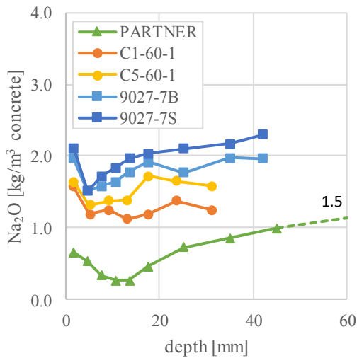
Fig. 9 : The Na 2 O-profiles (in kg/m 3 concrete) in function of the depth of the exposed surface (in mm) obtained by CWE for the examined samples. The 1.5 kg/m 3 Na 2 O indicated in the graph reflects the content determined on a section taken at a depth of approx. 100 mm-150.
