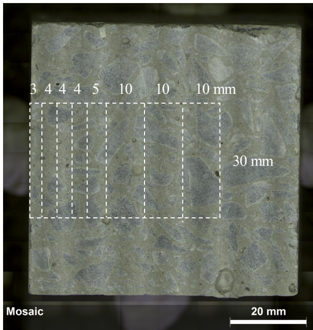
Fig. 4 : Mosaic image of the C5-60-1 sample taken with the \mu XRF. The white dotted lines indicate the sections mapped with the \mu XRF to obtain the alkali metal profiles. The numbers indicate the width and height of the sections taken.
