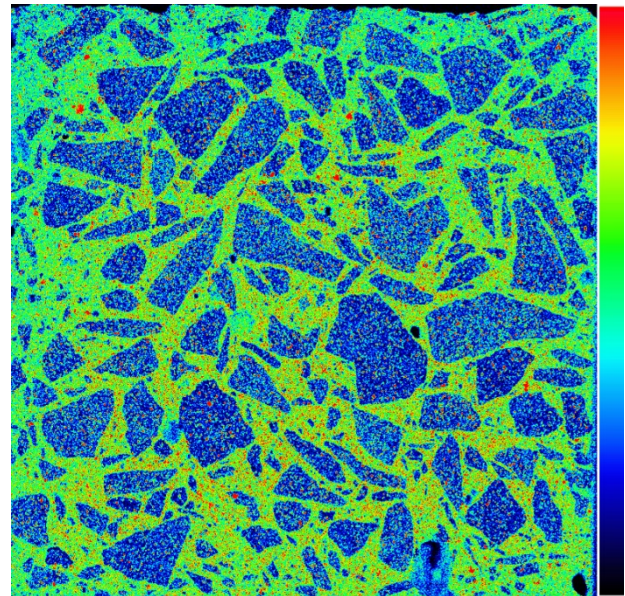
Fig. 10 : K-map of a sawn concrete surface of the C5-60-1 sample. The closer the color is to red the higher is the relative content of K. The dimensions of the sample are 70x70 mm.
