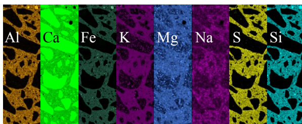
Fig. 5 : Elemental maps determined with the \mu XRF of section 30-40 mm of sample C5-60-1.
