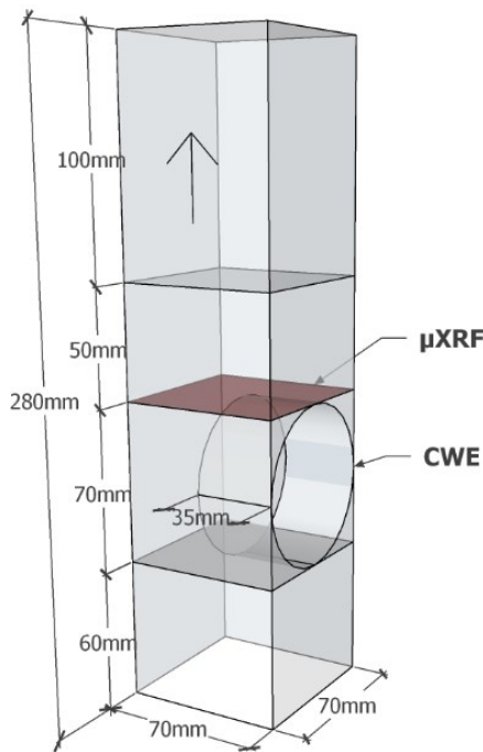
Fig. 3 : Sampling from prism C1-60-1 and C5-60-1.
