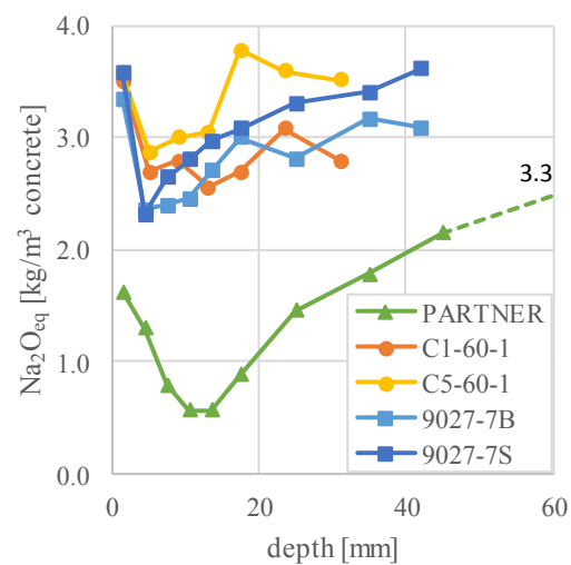
Fig. 7 : The \text{Na}_2\text{O}_{\text{eq}} -profiles (in \text{kg}/\text{m}^3 ) concrete in function of the depth of the exposed surface (in mm) obtained by CWE for the examined samples. The 3.3 \text{ kg}/\text{m}^3 \text{Na}_2\text{O}_{\text{eq}} indicated in the graph reflects the content determined in a section taken at a depth of approx. 100 mm-150.
