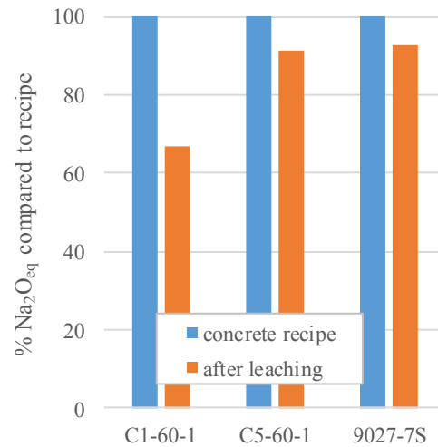
Fig. 16 : The % \text{Na}_2\text{O}_{\text{eq}} left in the concrete after leaching compared to the alkali content initially in the concrete (concrete recipe, Table 2).
