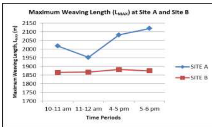
Figure 3. Graph of maximum weaving length at sites
