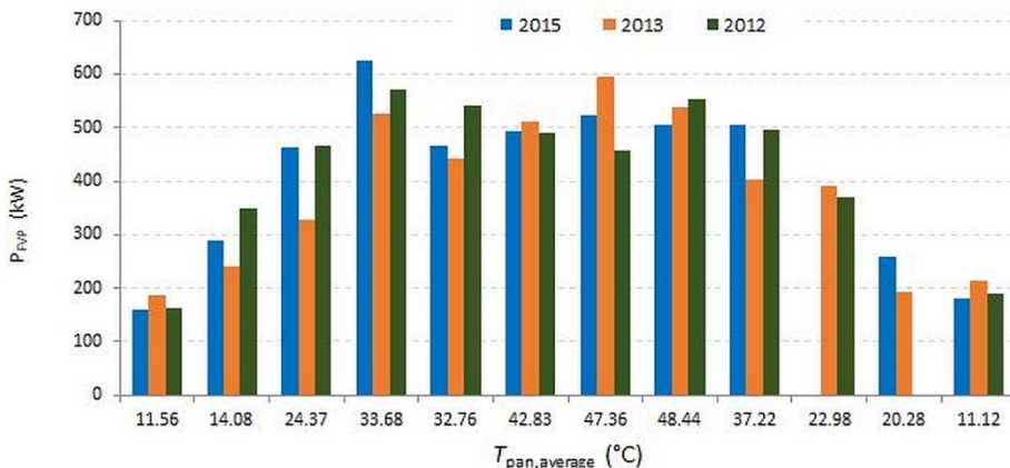
Fig. 3. Comparison of average monthly PV power over the reference period.
