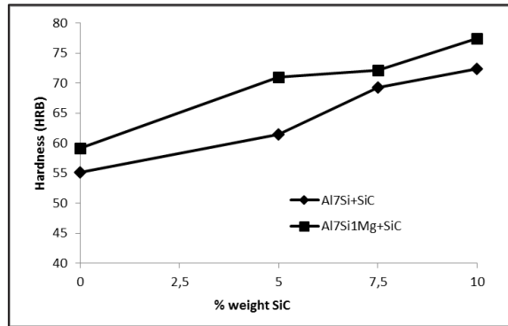
Fig. 3. The hardness of Al7Si and Al7SiMg composites
