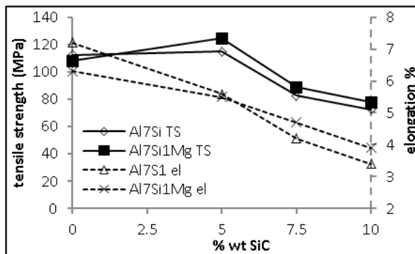
Fig. 4. The tensile strength and elongation of Al7Si and Al7SiMg composites.
