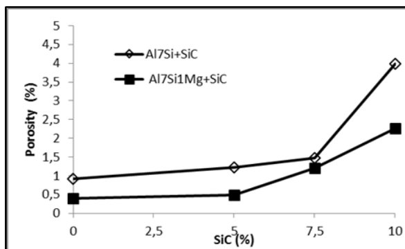
Fig. 5. The porosity of Al7Si and Al7SiMg composites
