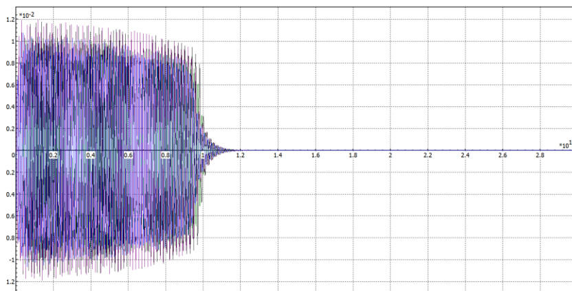
Fig. 4. Horizontal lateral displacement of wheelsets (wheel profile in accordance with GOST 9036). Horizontal axis: time [s], Vertical axis: wheelset lateral displacement [m]
