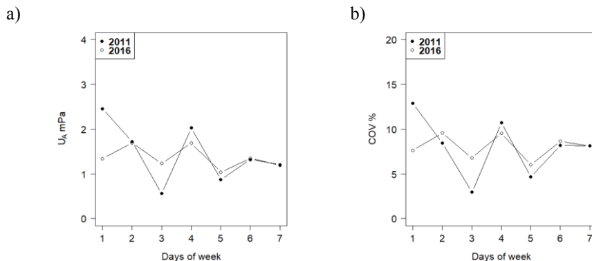
Fig. 4. Comparison of the values of a) sound pressure measurement uncertainty – Type A evaluation, b) the COV , recorded in 2011 and 2016.
