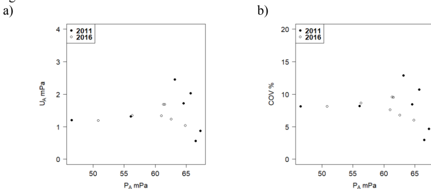
Fig. 5. Average value of the RMS sound pressure versus a) sound pressure measurement uncertainty – Type A evaluation, b) the COV , for the measurement data of 2011 and 2016.
