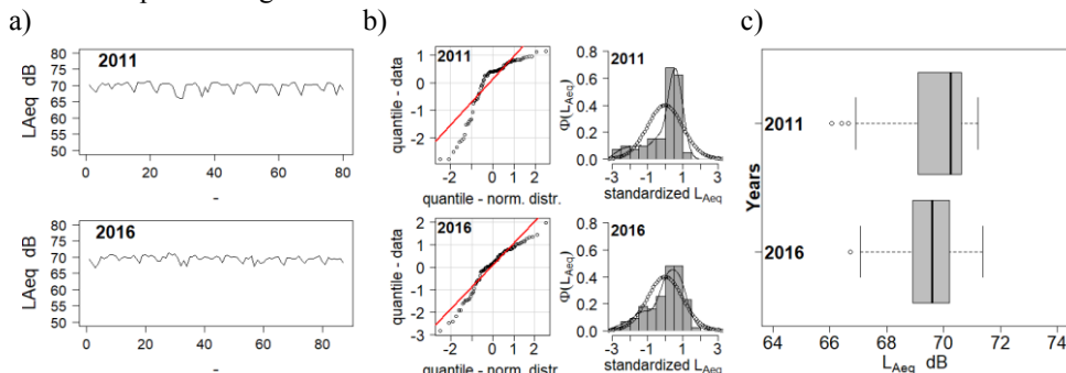
Fig. 1. Equivalent sound level results from the terminal in Popiełuszki Avenue recorded in 2011 and 2016 for all 24-hour measurement periods; a) equivalent sound level variations and the corresponding; b) quantile plots and histograms with the function of probability density distribution for the standardized data, c) box plots.
