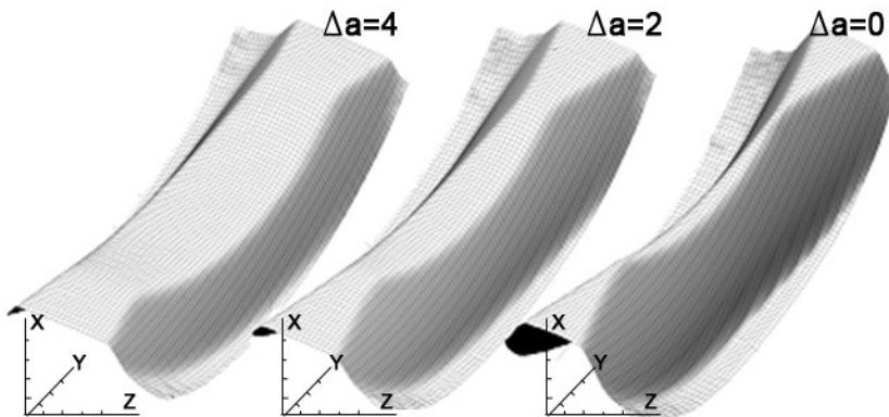
Fig. 4. The radial toothing cutting method – the parameter \Delta a defines the indentation; number of teeth, 31; module, 3 mm; inner diameter, 105 mm
