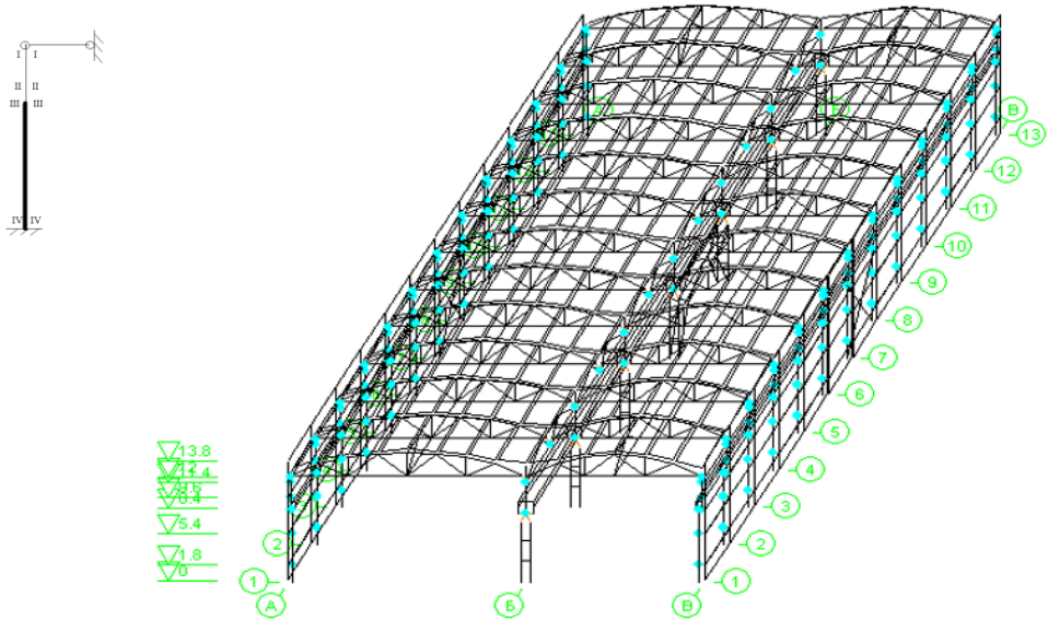
Fig.3. 3D calculation model of the frame
