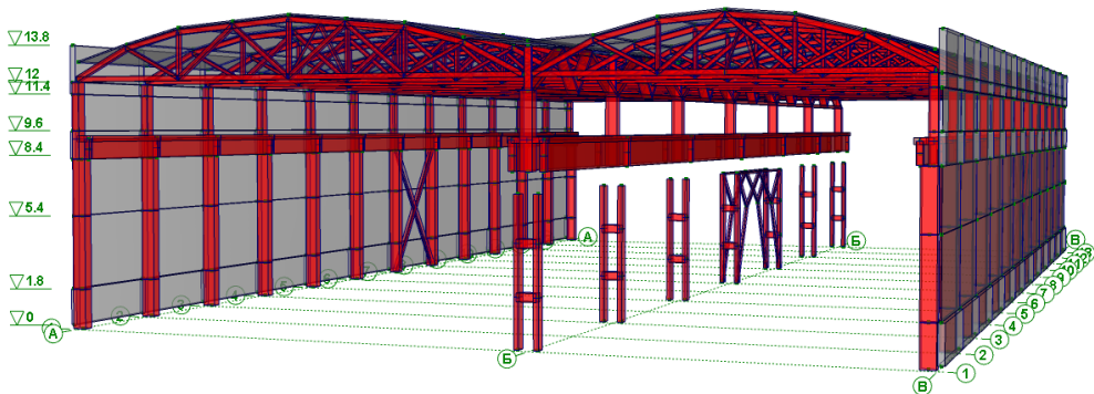
Fig.2. Calculation model
