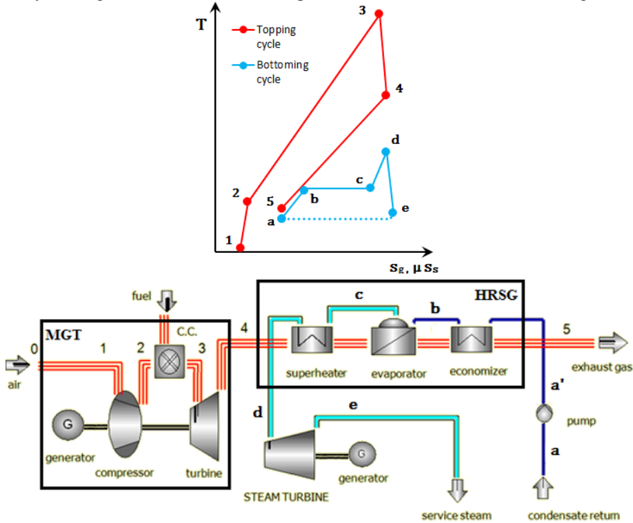
Fig. 1. Schematic representation of the cogeneration system
