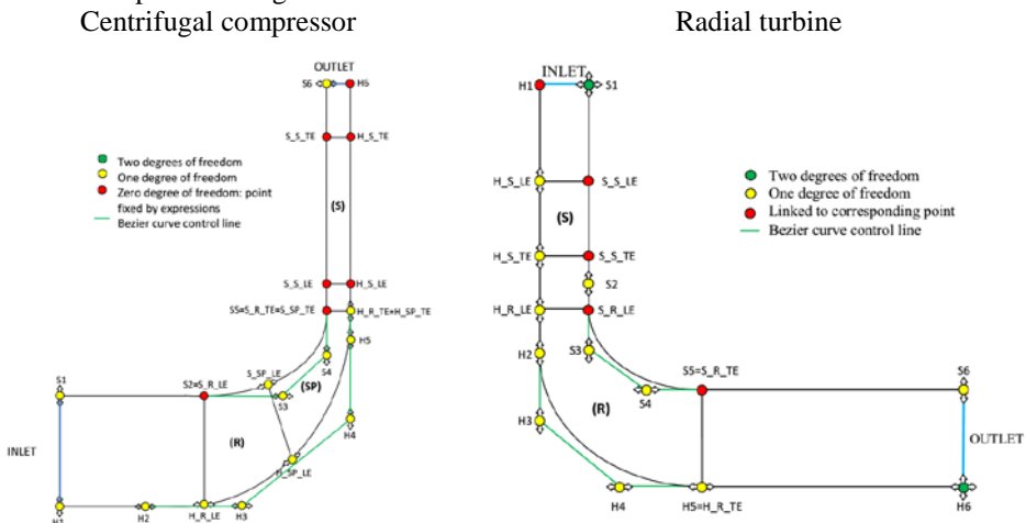
Fig. 4. Compressor and turbine geometrical parameterization
