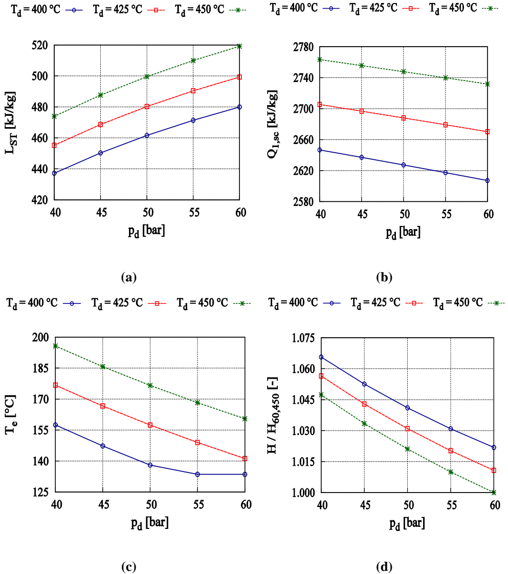
Fig. 2. Influence of p_d and T_d on: (a) L_{st} , (b) Q_{1,sc} , (c) T_e , (d) H/H_{60,450}
