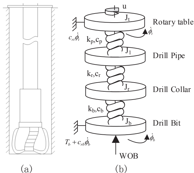
Fig. 1. The schematics of (a) the drill-string and (b) the simplified physical model of the drill-string system
