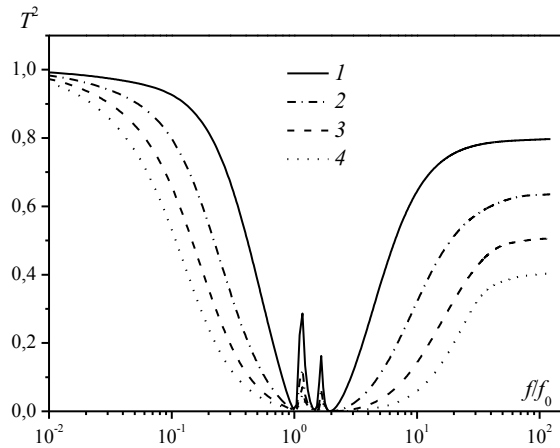
Fig. 3. Coefficient of sound transmission through a bubbly screen at different layer thickness.
