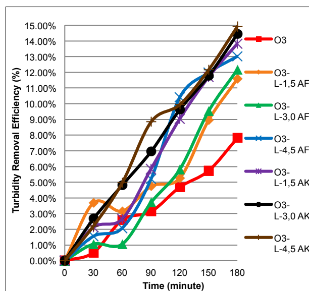
Figure 5. Turbidity Removal Efficiency.
