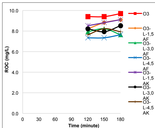
Figure 4. Residual Ozone Concentration.
