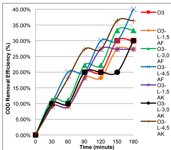
Figure 7. COD Removal Efficiency.
