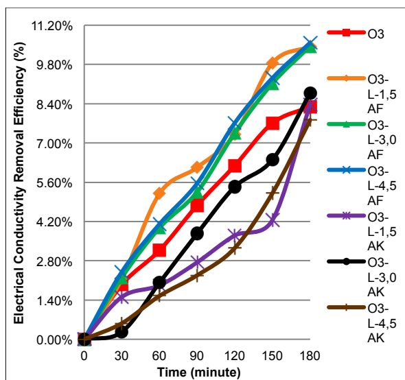
Figure 6. Electrical Conductivity Removal Efficiency.
