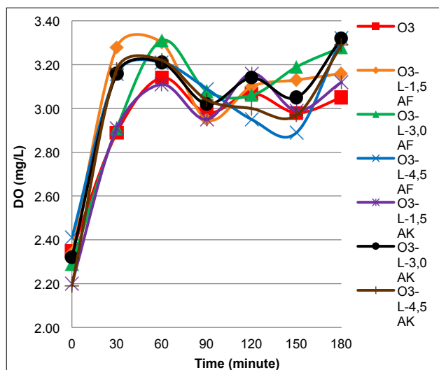
Figure 3. Dissolved Oxygen by Time.
