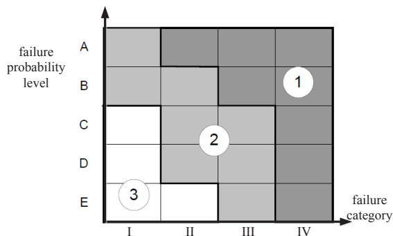
Fig. 1. Characteristics of the severity of failure consequences in a power supply system.
