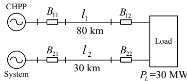
Fig. 2. Scheme of the power supply system.
