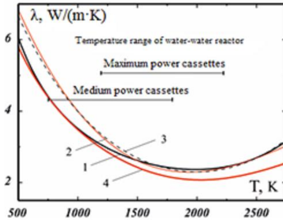
Fig. 1. Comparison of approximations using the thermal conductivity UO_2 : 1 – theoretical dependence (3) of work [12]; 2 – empirical formula (4), [12]; 3 – formula (5); 4 – Fink-Ronchi ratio (6).
