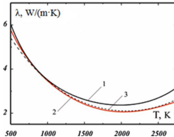
Fig. 2. Updating of approximation using the thermal conductivity UO_2 : 1 – theoretical dependence (3) of work [11]; 2 – Fink-Ronchi ratio (6); 3 – formula (7).
