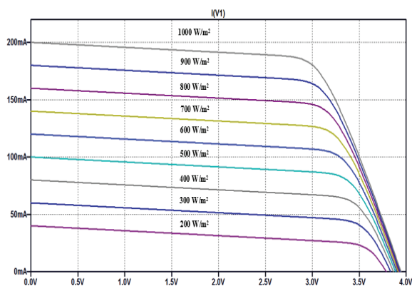
Fig. 8. Solar Irradiation levels from 200 W/m 2 to 1000 W/m 2 at 25 °C
