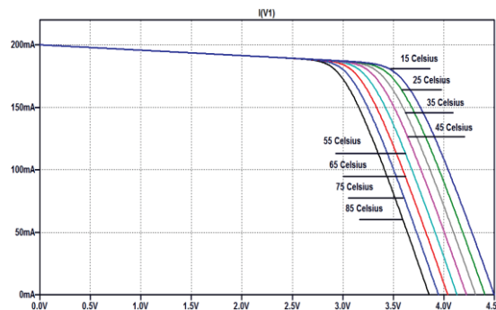
Fig. 9. I – V Characteristics for Temperature variation between 15 °C to 85 °C at 1000 W/m 2
