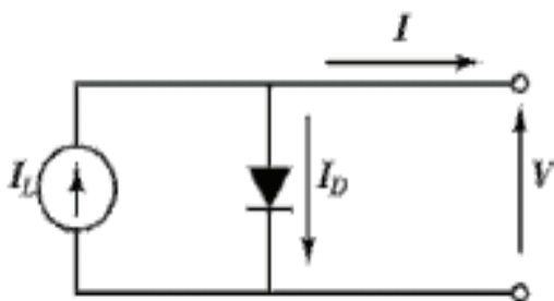
Fig. 2. Ideal Single Diode Model (1M3P)
