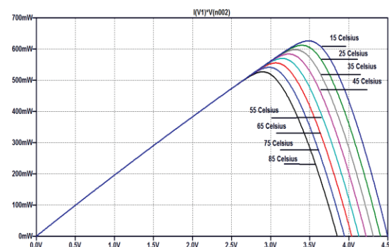
Fig. 10. P – V Characteristics for Temperature variation between 15 °C to 85 °C at 1000 W/m 2
