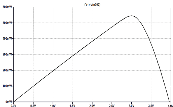
Fig. 7. P – V curve of Solar Equivalent Circuit of iXolar SolarMD SLMD481H08L
