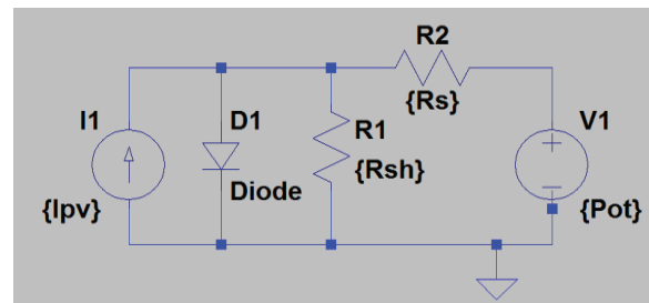
Fig. 5. Single diode Equivalent circuit for iXolar SolarMD SLMD481H08L
