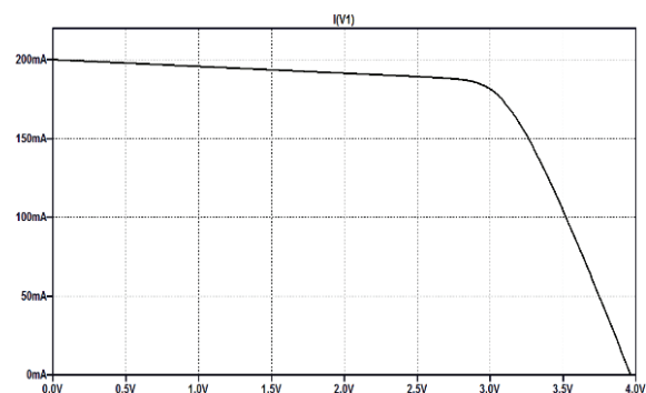
Fig. 6. I – V curve of Solar Equivalent Circuit of iXolar SolarMD SLMD481H08L
