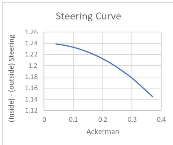
Figure 3. Steering Curve
