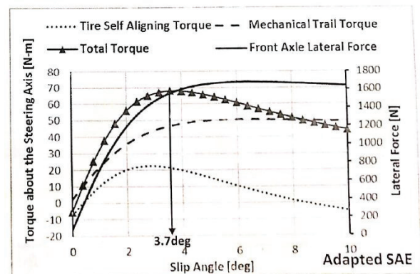
Figure 6. Steering torque vs slip angle (30 mm Mechanical trail)
