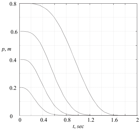
Fig. 8. Dynamics of a ball under a fuzzy-modal control.
