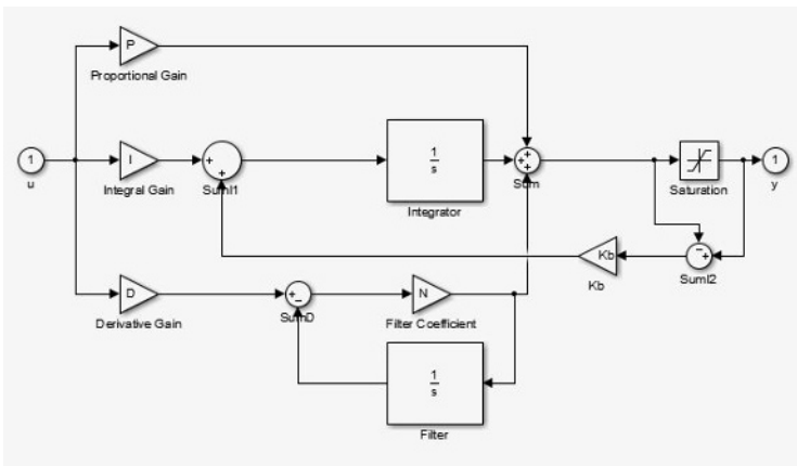
Fig. 1. Back-Calculation algorithm.
