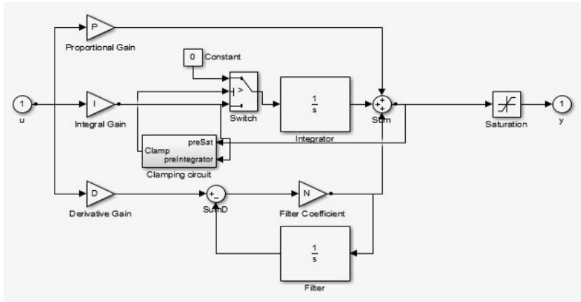
Fig. 2. Clamping algorithm.
