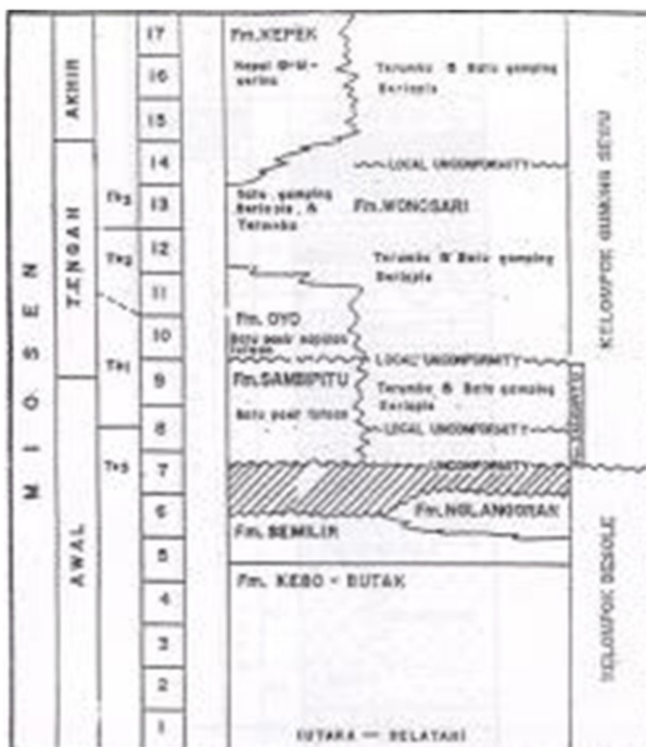
Fig.2. Stratigraphy Southern Mountains (Suyoto, 1992)
