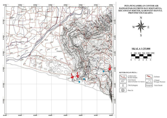
Fig.3. Sampling Hot Water Spring in Parangwedang
