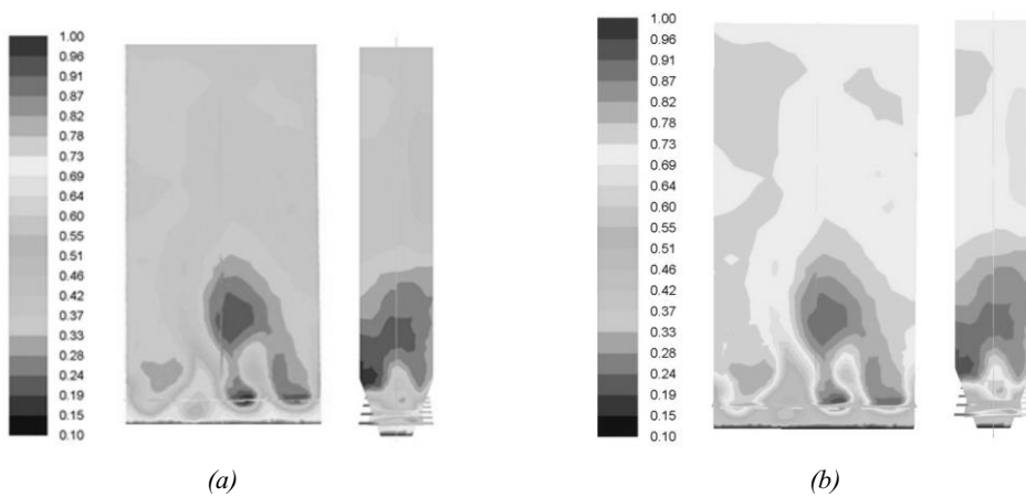
Fig. 4. Height variation of the furnace estimated phases concentration values in vertical cross-section at 5 m/s of airflow supply from below: (a) particles; (b) air
