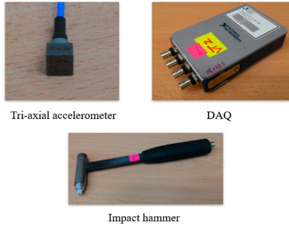
Fig. 3. Equipment used for EMA.
