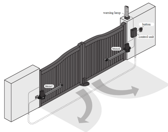
Figure 3. Example of construction of a remotely controlled gate with two drivers [5].
