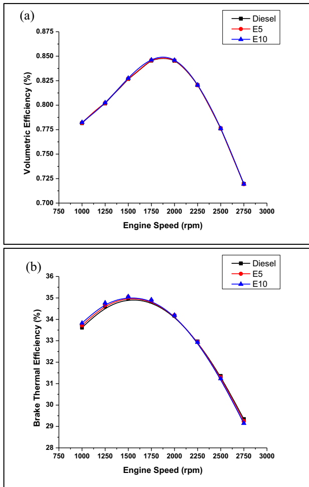
Figure 3. (a) Volumetric efficiency (b) Brake Thermal Efficiency against different engine speed
