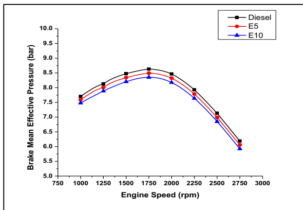
Figure 6. Brake mean effective pressure against engine speed
