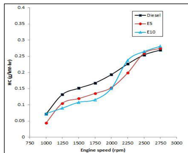
Figure 8. Hydrocarbon against engine speed
