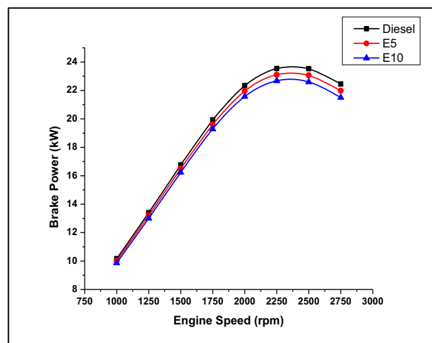
Figure 5. Brake power result against engine speed
