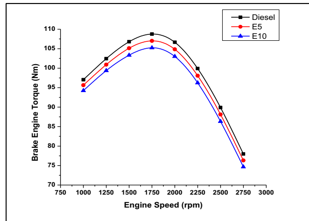
Figure 4. Brake engine torque against engine speed
