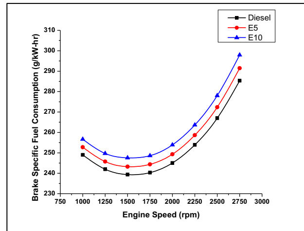
Figure 7. Brake specific fuel consumption against engine speed
