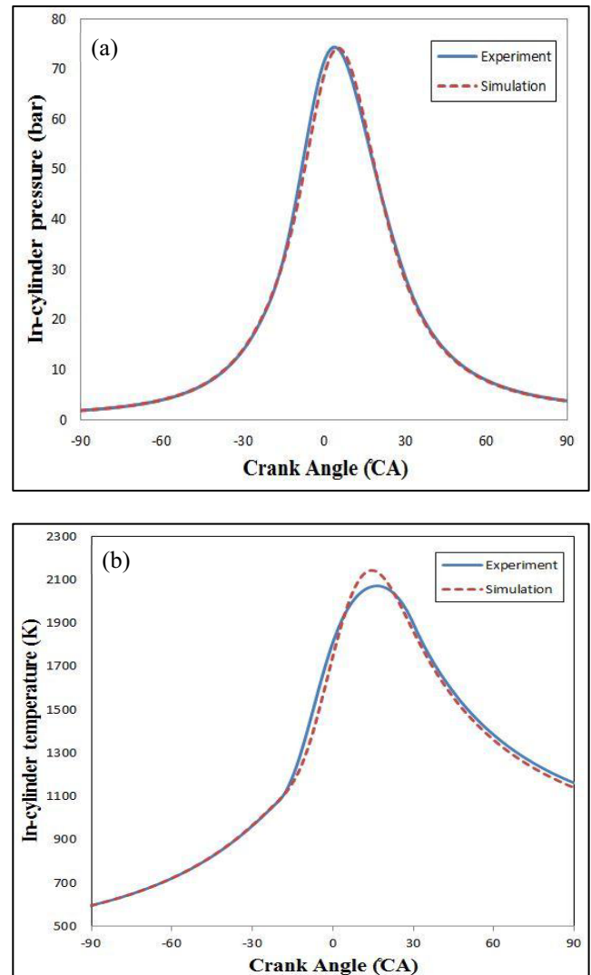
Figure 2. A comparison of simulated and experimental in-cylinder pressure (a) and temperature (b) under full load at 1500 rpm engine speed.
