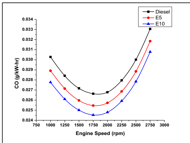
Figure 9. Carbon monoxide against engine speed
