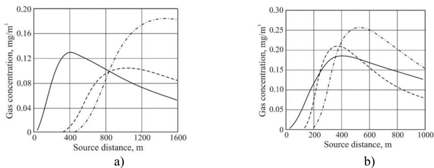
Fig. 1. Distribution of the ground-level concentration of gaseous pollutants along the plume centre-line at critical wind velocities corresponding to favorable (a) and unfavorable (b) weather conditions:— — and — · — · — calculation by the Paskvill's model ( z_0 = 10 cm and 1 cm);—— - calculation by the OND-86 technique.
