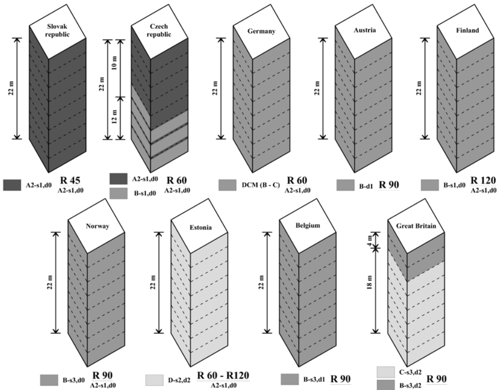
Figure 5. Mutual comparison of façade requirements in selected European countries on buildings with height till 10 and till 22 m.
