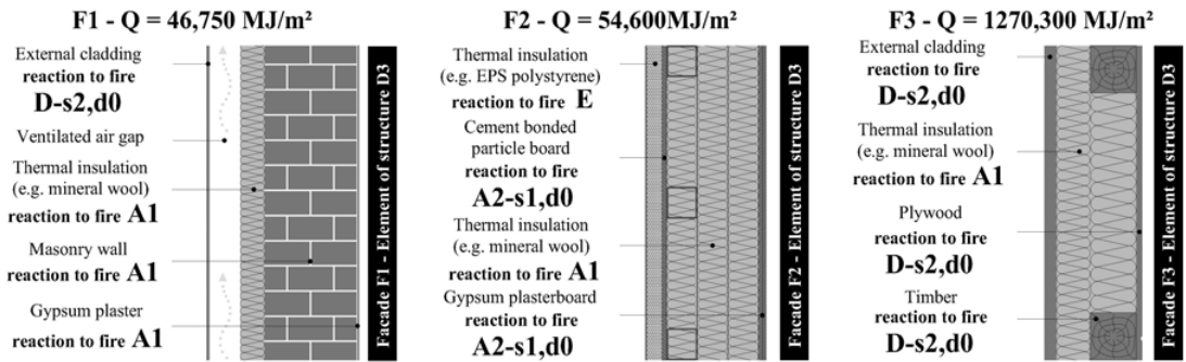
Figure 4. Total amount of heat release from façade in various material composition.
