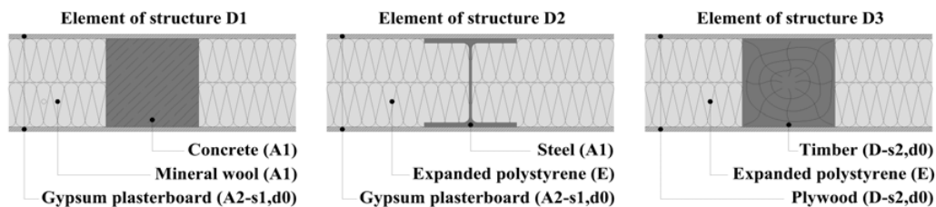
Figure 1. Elements of structure.
