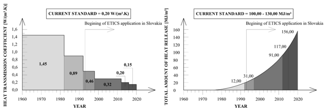
Figure 3. Increase in demands on the heat transmission coefficient value and total amount of heat release from façade [11].
