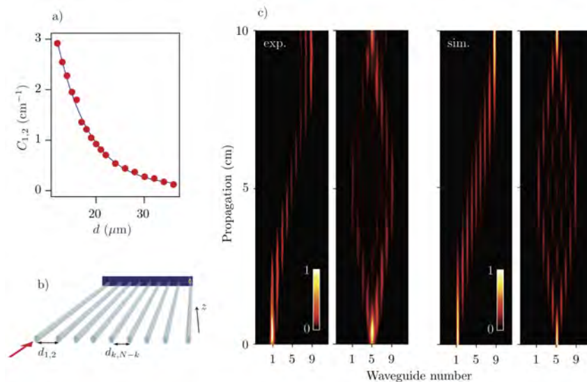
Fig. 1: a) Coupling strength C versus waveguide separation d . b) Sketch of the photonic lattice with judiciously engineered couplings. c) Light propagation in an array of N = 9 waveguides with coupling distribution given by eq. (1) when the first and fifth waveguide are initially excited. Left panels: Experiments. Right panels: Simulations. Adapted from [7]
