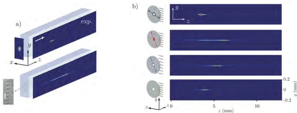
Fig. 2: Observation and tailoring of a lattice filament. a) top: A standard filament, bottom: a lattice filament. The yz image size is 0.4 \times 13 mm. b). Modification of the lattice period and input polarisation allows to tailoring the lattice filament attributes. Adapted from [10]
